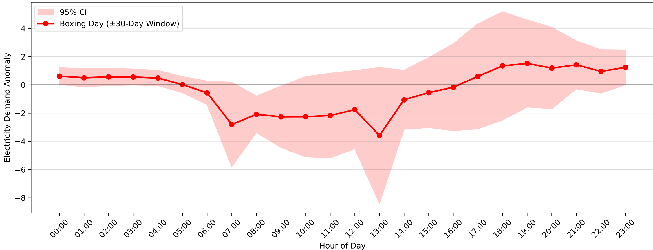
Broadmeadow Demand Anomaly: Boxing Day (2004–2017, \pm 30 -Day Window)
